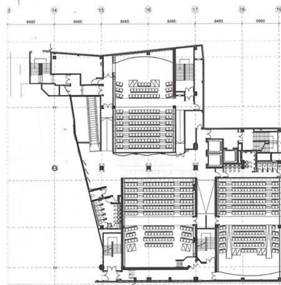
Level 10 Floor Plan
