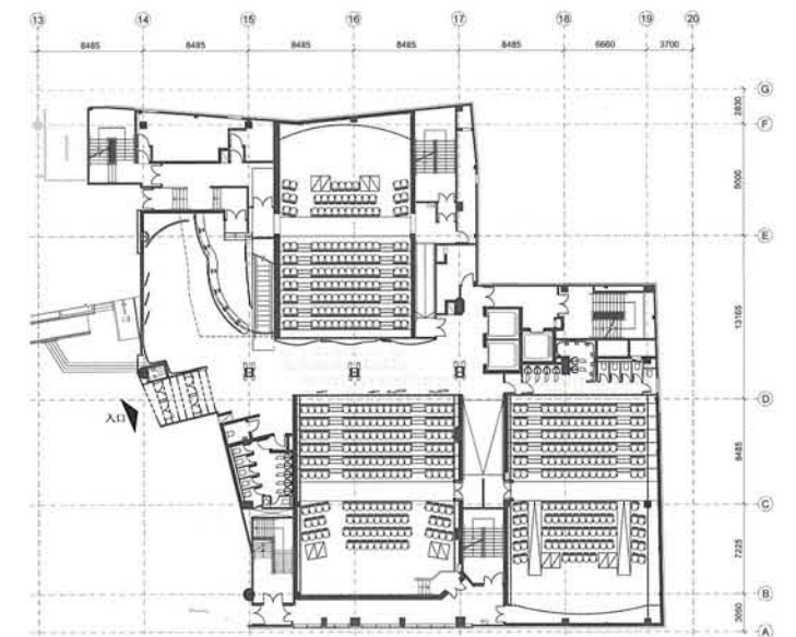
Level 8 Floor Plan
